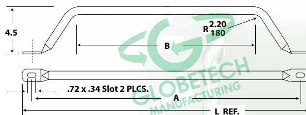
Stainless Steel Tracker Bar
